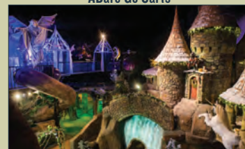
Wizard Quest
